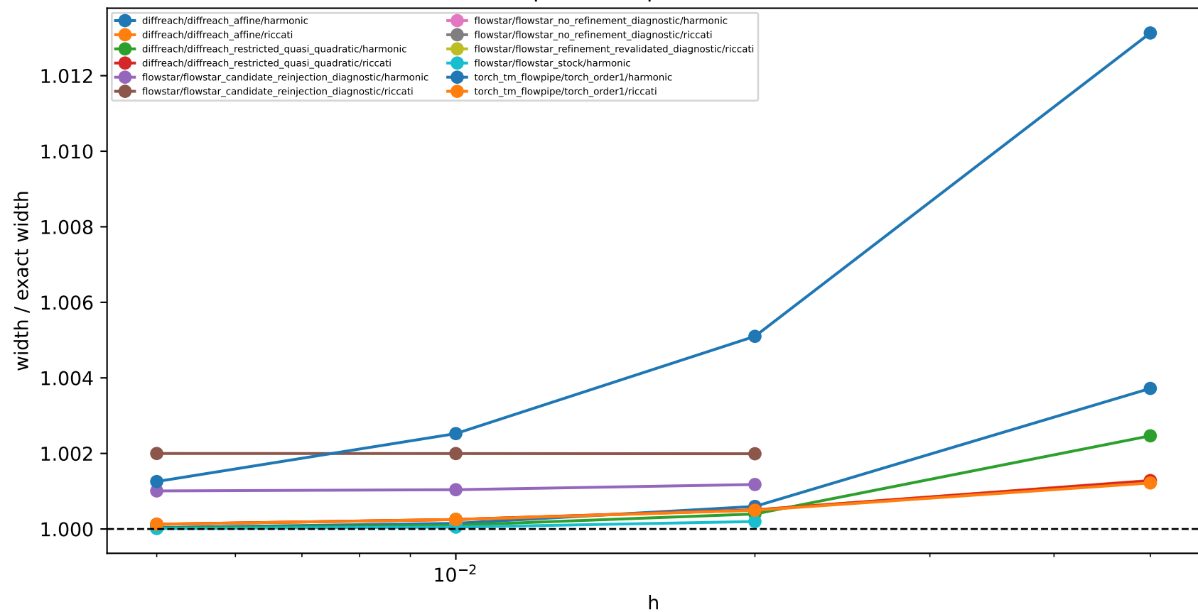
one step raw endpoint inflation vs h
