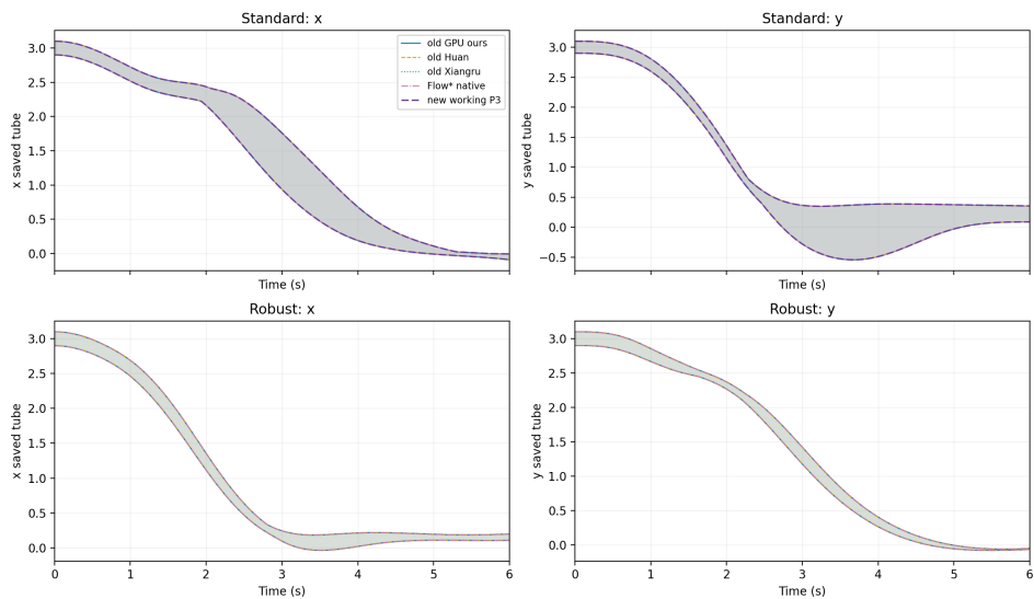
NAV saved flowpipe x/y projections
