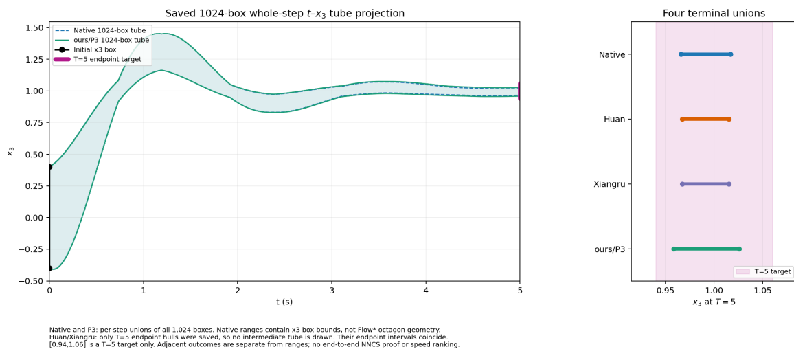
ARCH-COMP 2026 paper-equation QUAD — saved intervals, full initial partition
