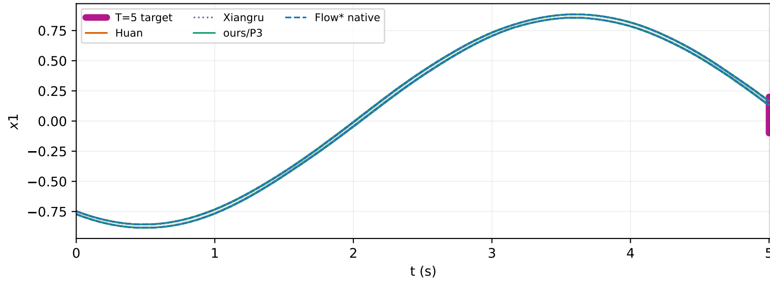
Saved whole-step x_1 tube ( 500 \times 0.01 s)
