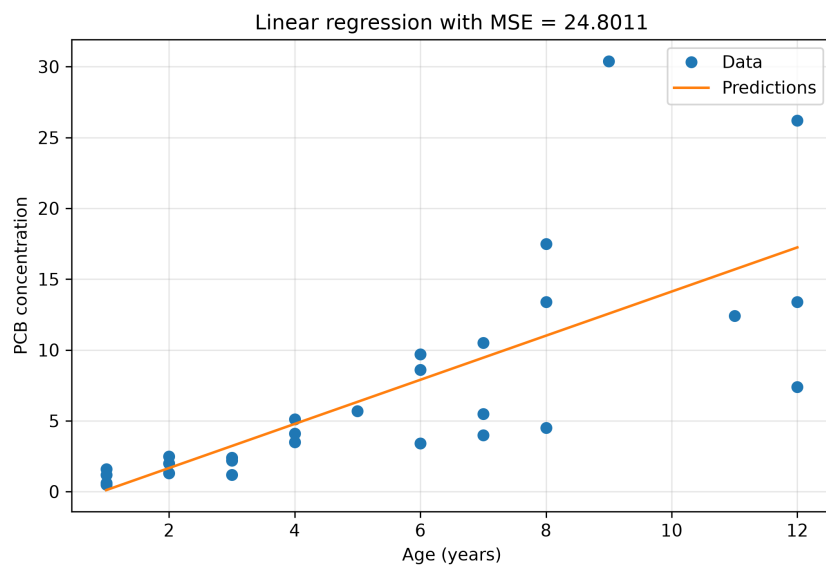
Figure 6: Linear regression
