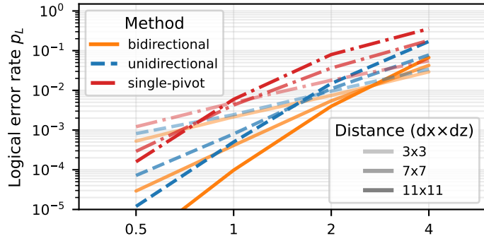
|0\rangle state
