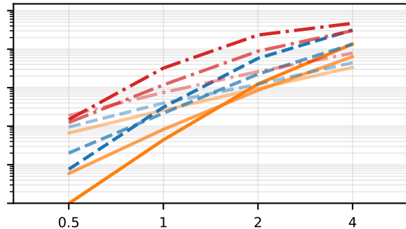
|+\rangle state
