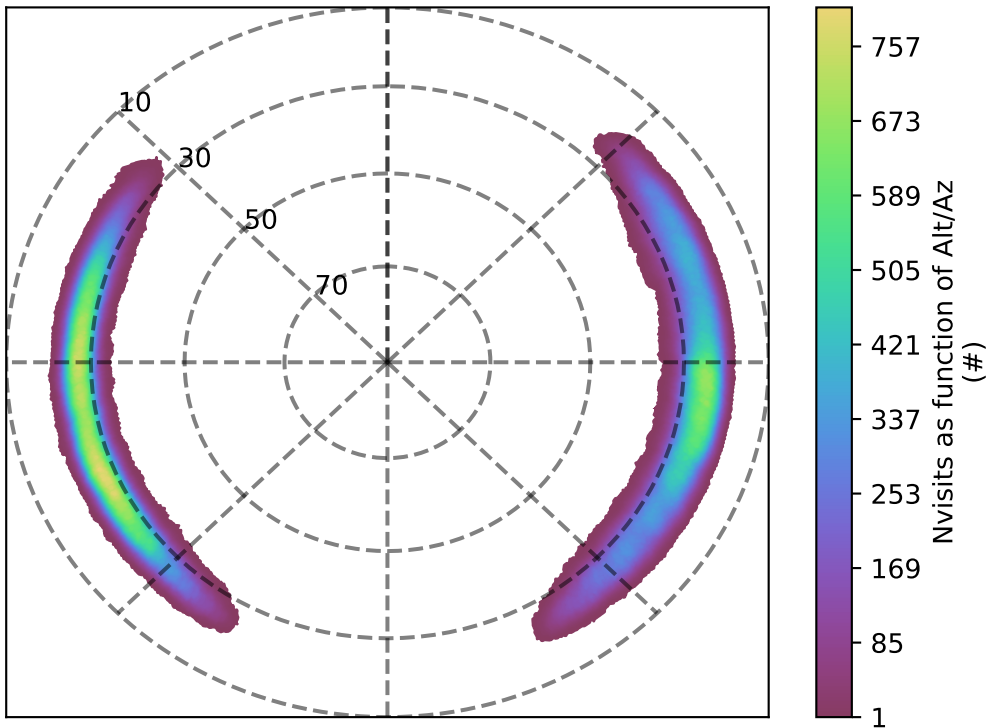
Twilight Earth-Interior (v4.3.1)
