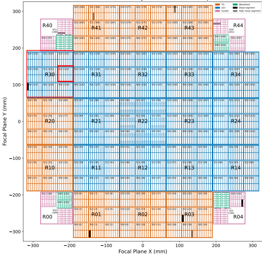
LSST Camera Focal Plane by Raft, Sensor, and Amplifier
