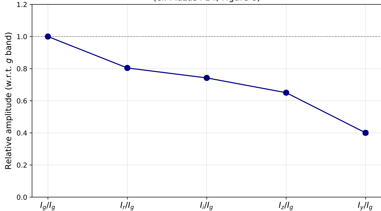
Detector 11 (R02_S02) -- Tree-ring amplitude vs band (cf. Plazas+14, Figure 8)
