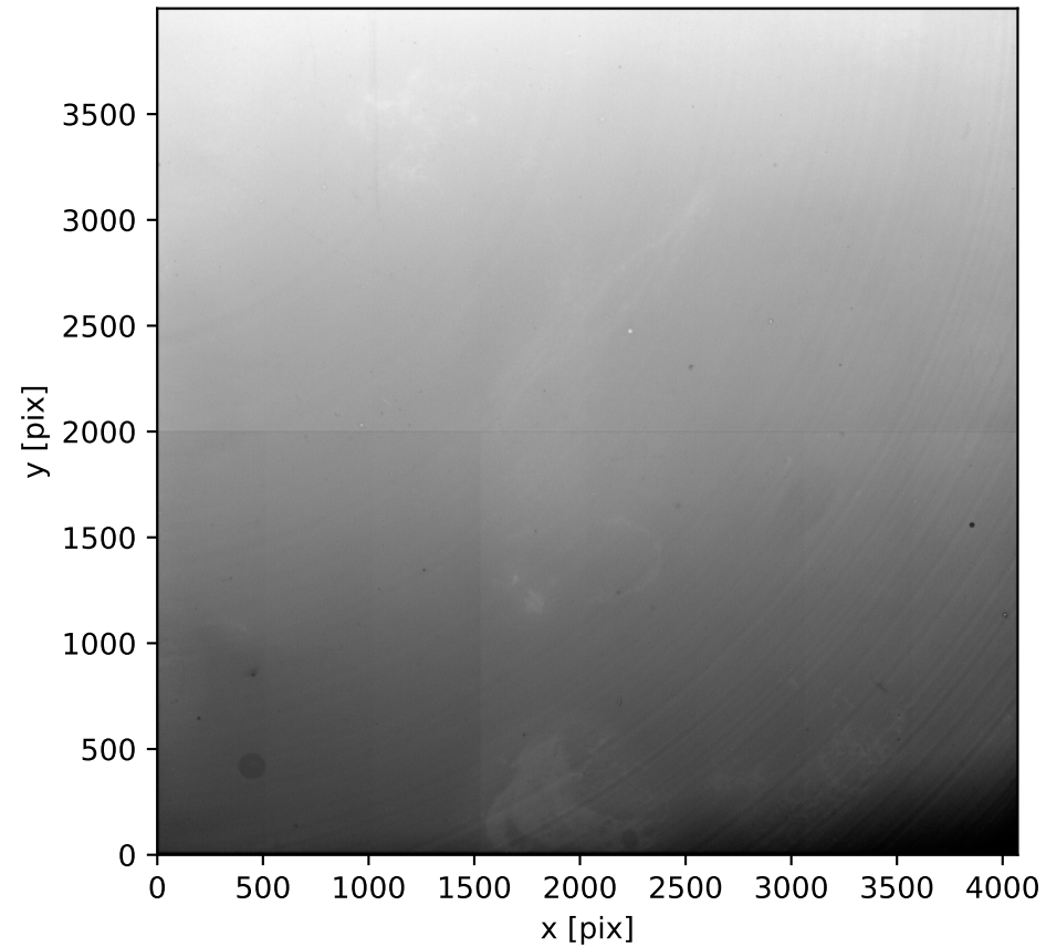
Detector 11, g-band
