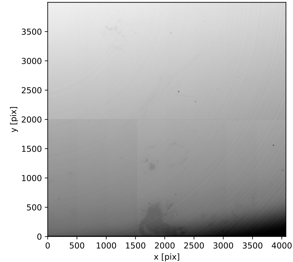
Detector 11, i-band
