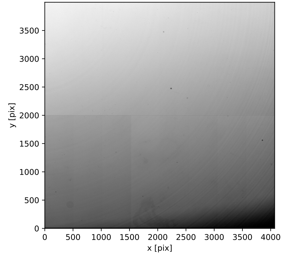
Detector 11, r-band
