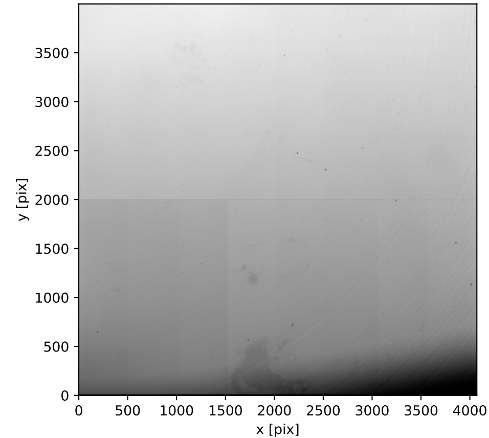
Detector 11, z-band
