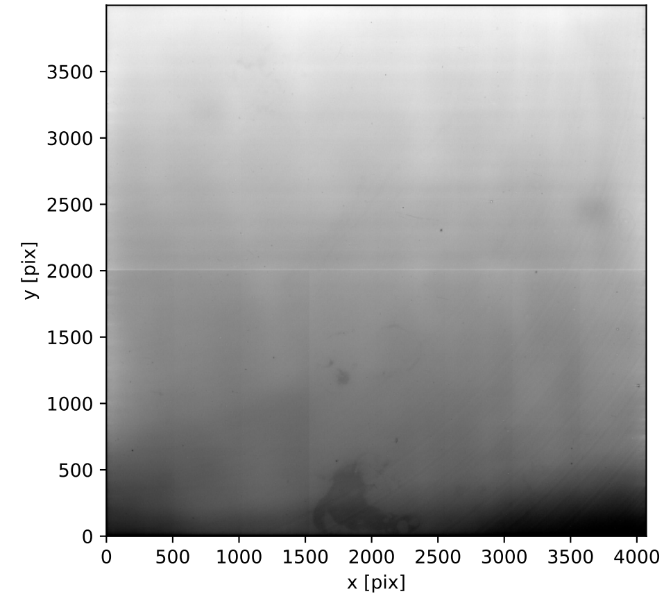
Detector 11, y-band
