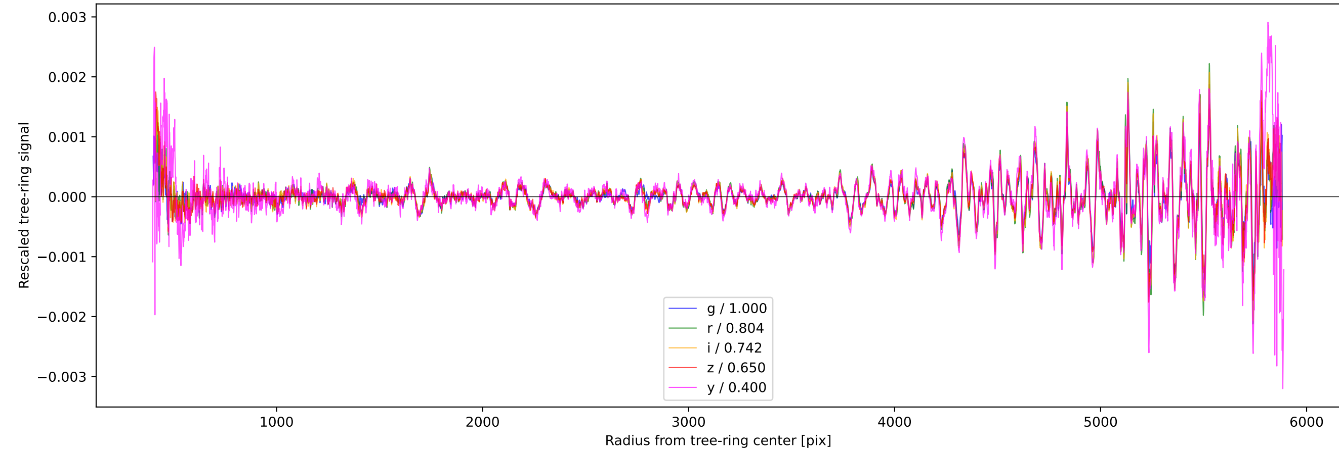
Profiles rescaled to g-band amplitude -- should overlap if in phase
