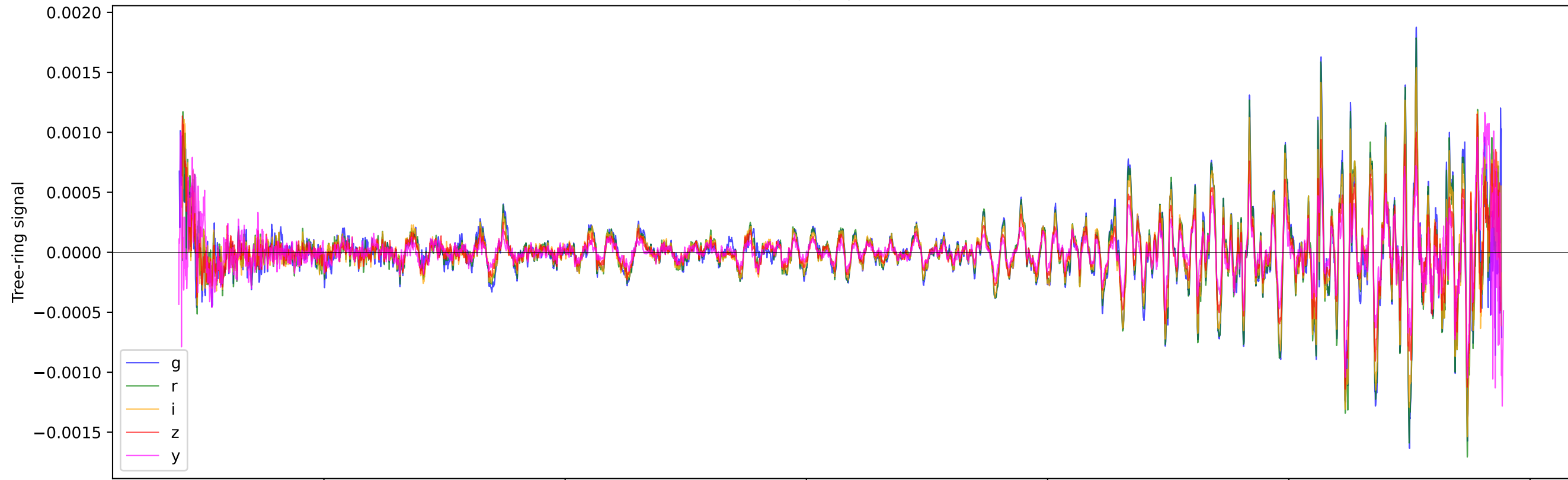
Profiles rescaled to g-band amplitude -- should overlap if in phase
