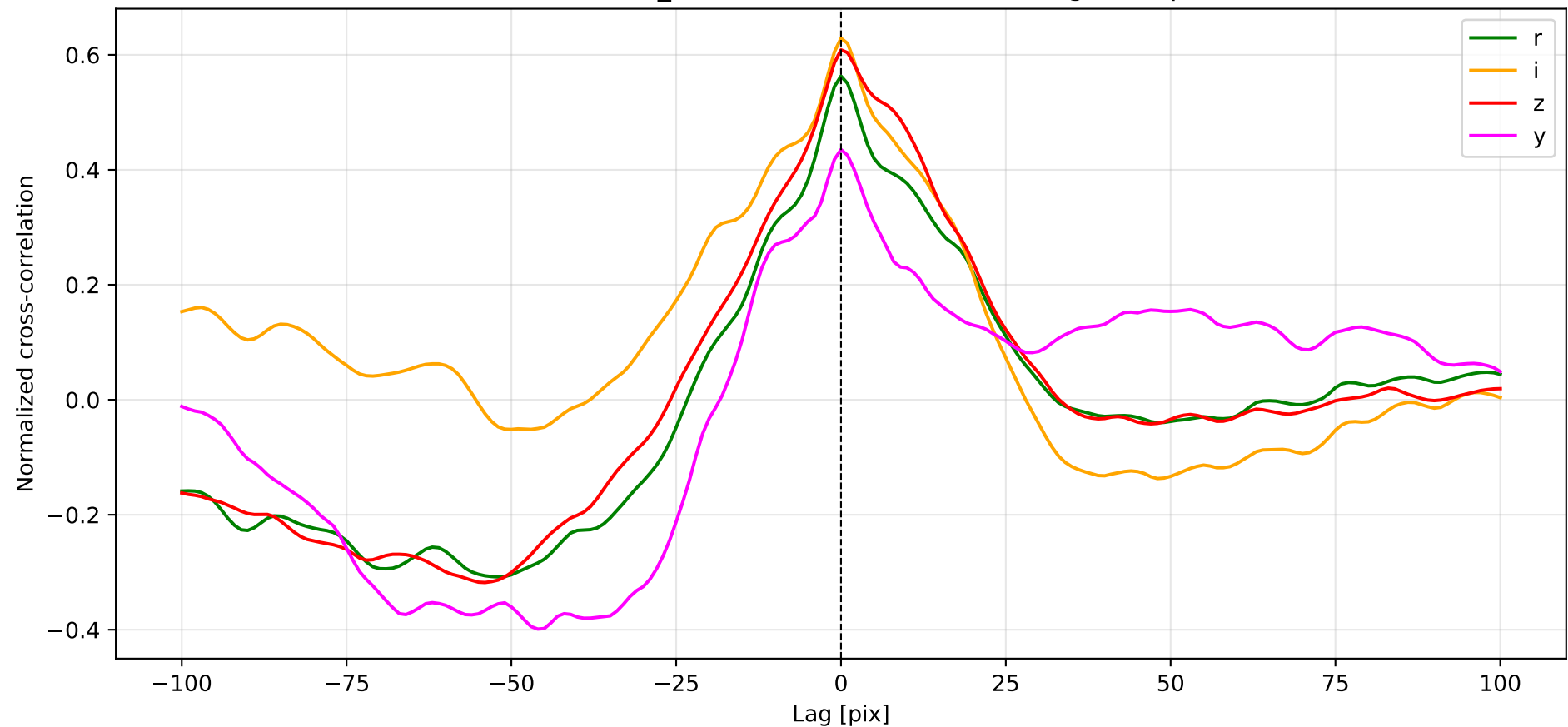
Detector 11 (R02_S02) -- Cross-correlation with g-band profile
