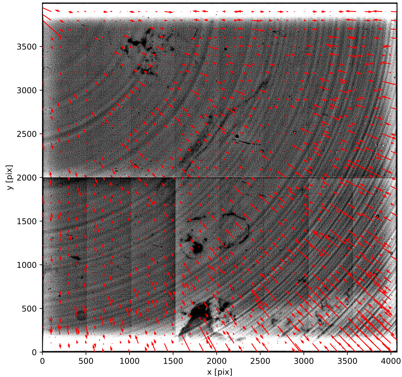
Predicted tree-ring astrometric displacement field
