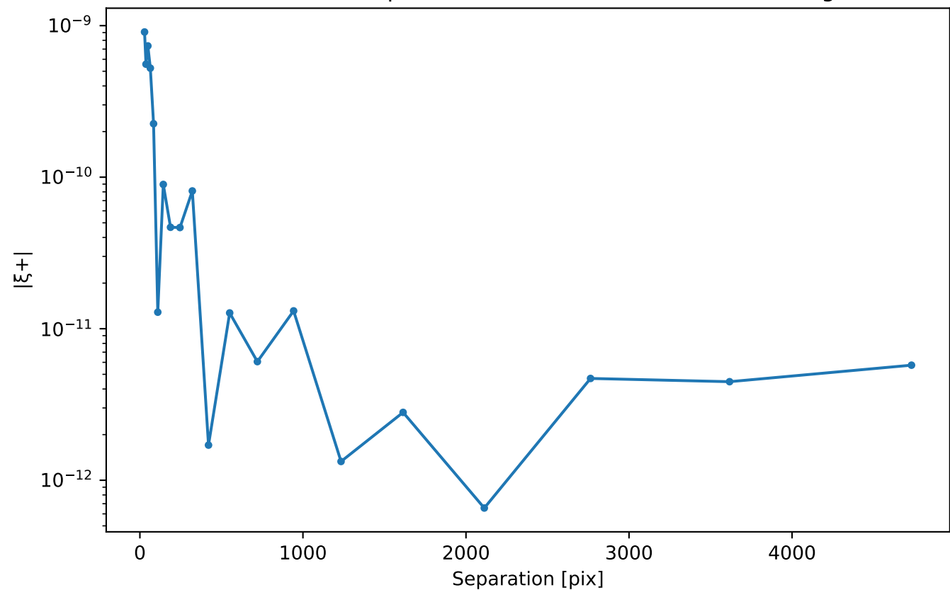
Detector-level spurious shear correlation from tree rings
