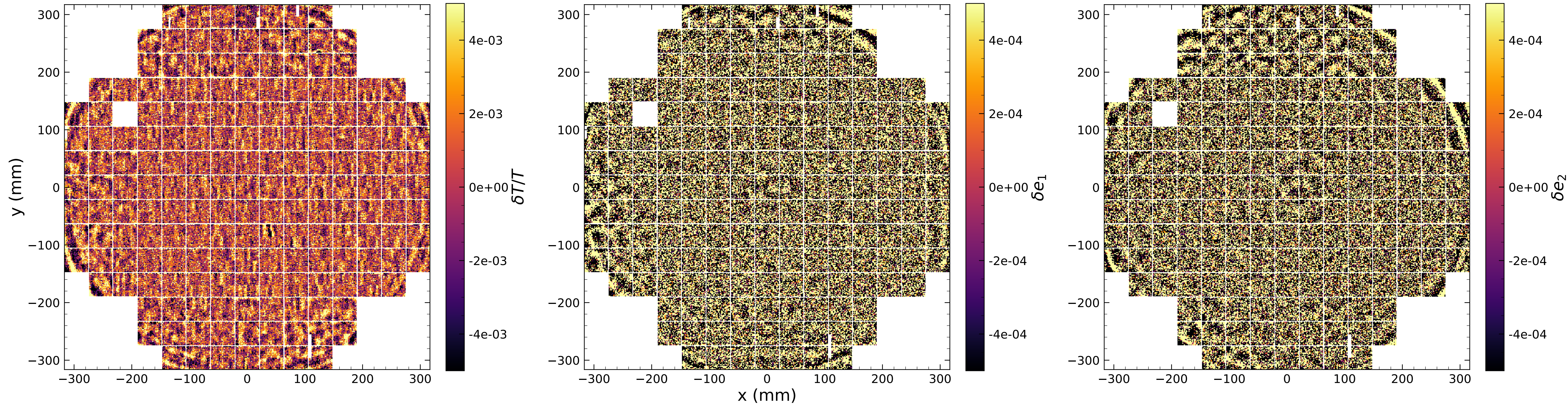
u-band
