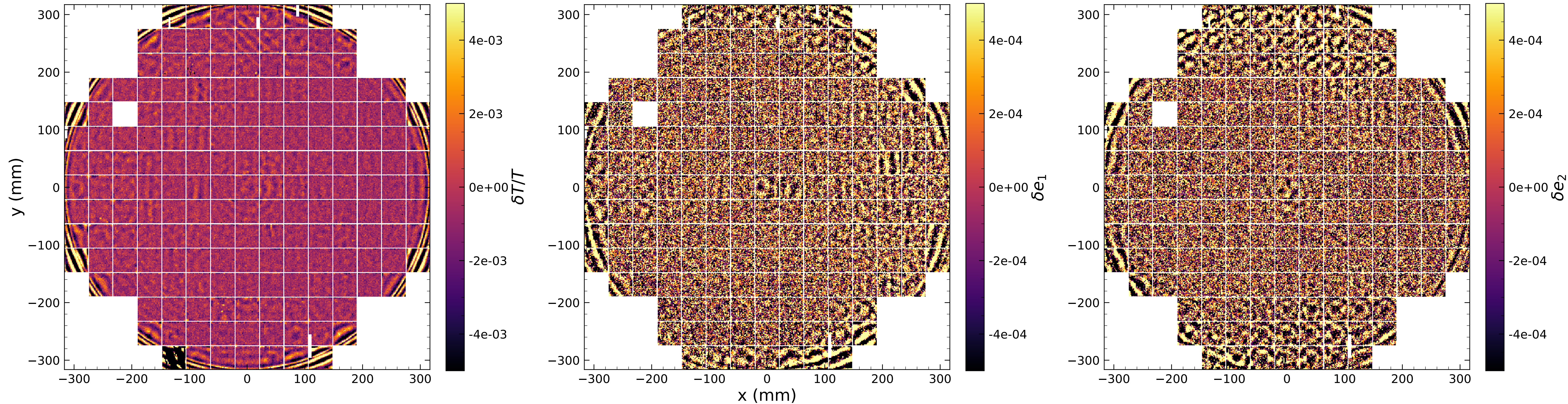
i-band
