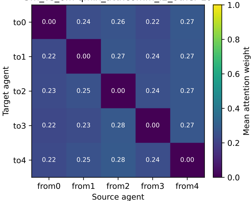
5m_vs_6m qmix_attncomm_l2_other L0
