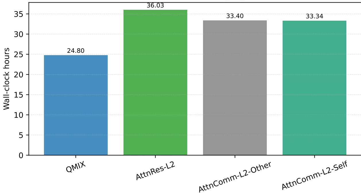
Training Time on 5m_vs_6m
