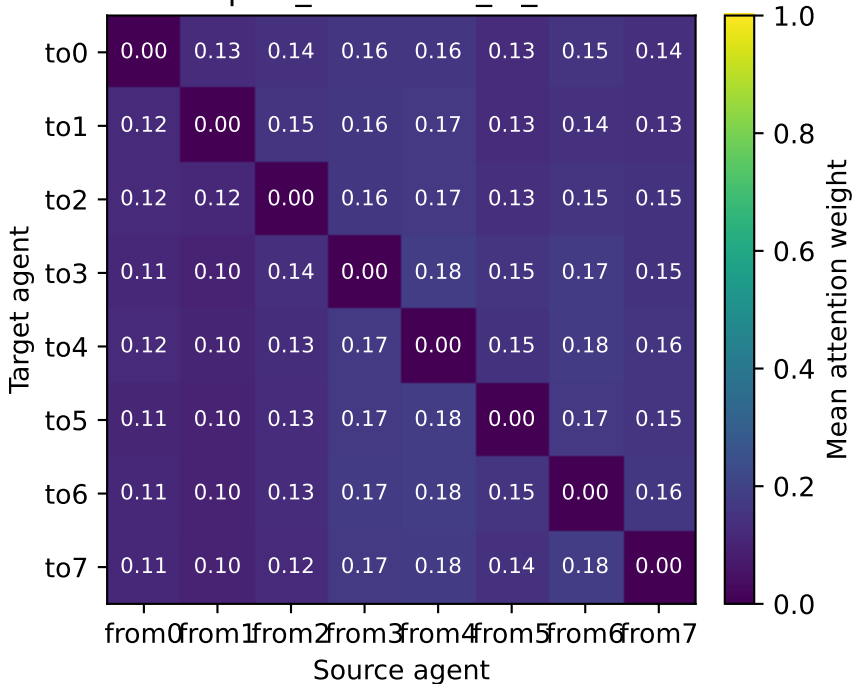
3s5z qmix_attncomm_l2_other L1
