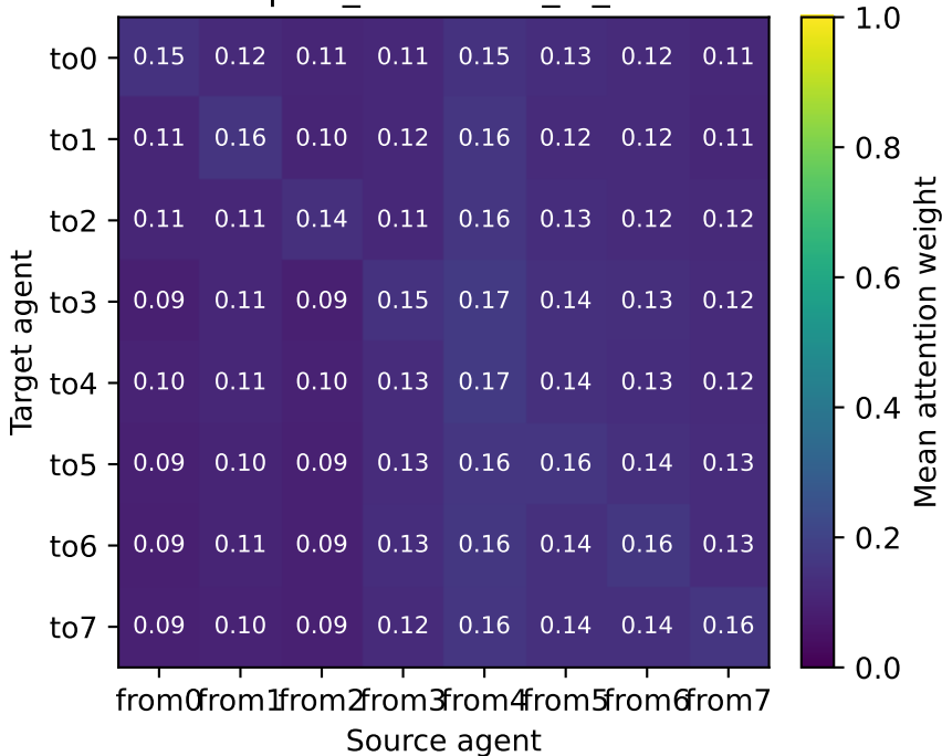
3s5z qmix_attncomm_l2_self L1
