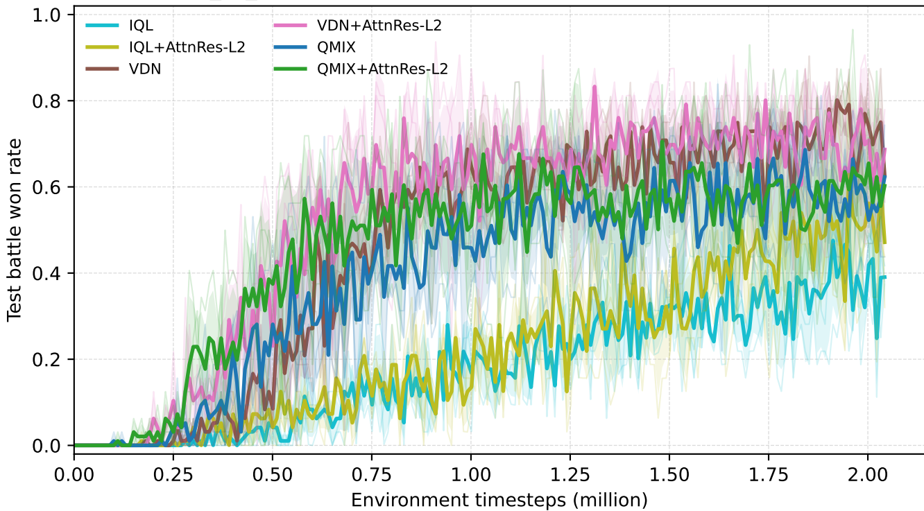
5m_vs_6m: Lightweight AttnRes-L2 Cross-Algorithm Check
