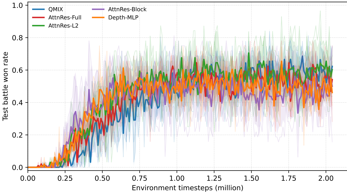
5m_vs_6m: QMIX Variants
