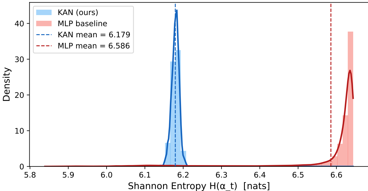
Activation Entropy Distribution: KAN vs MLP Temporal Gate
