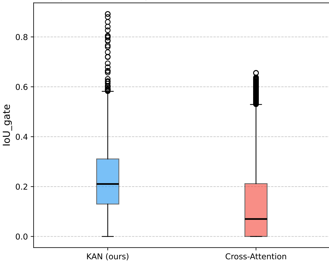
Spatial Gate Fidelity: KAN Decoder vs Cross-Attention
