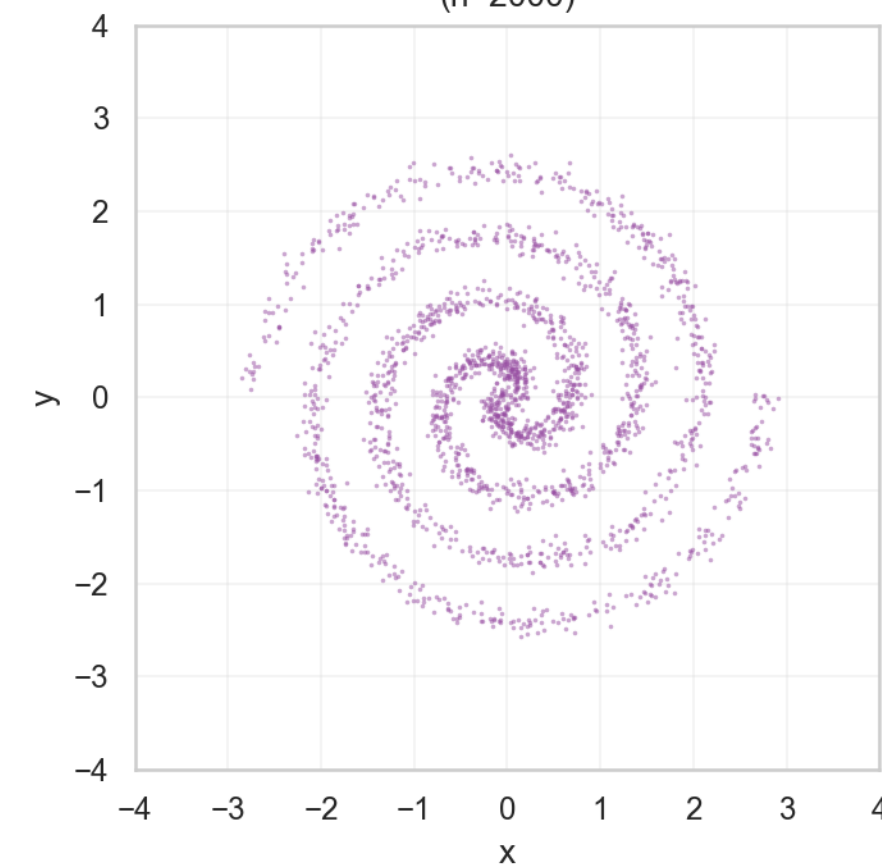
Spiral (n=2000)
