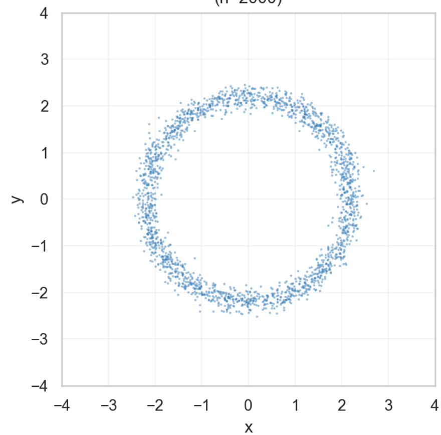
Ring (n=2000)
