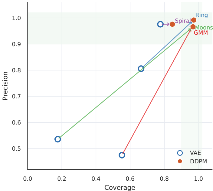
Precision-Coverage plane
