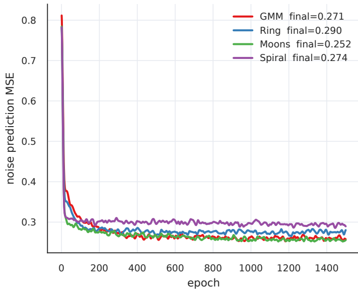
DDPM convergence
