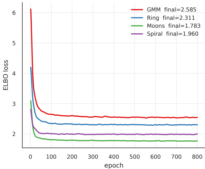
VAE convergence
