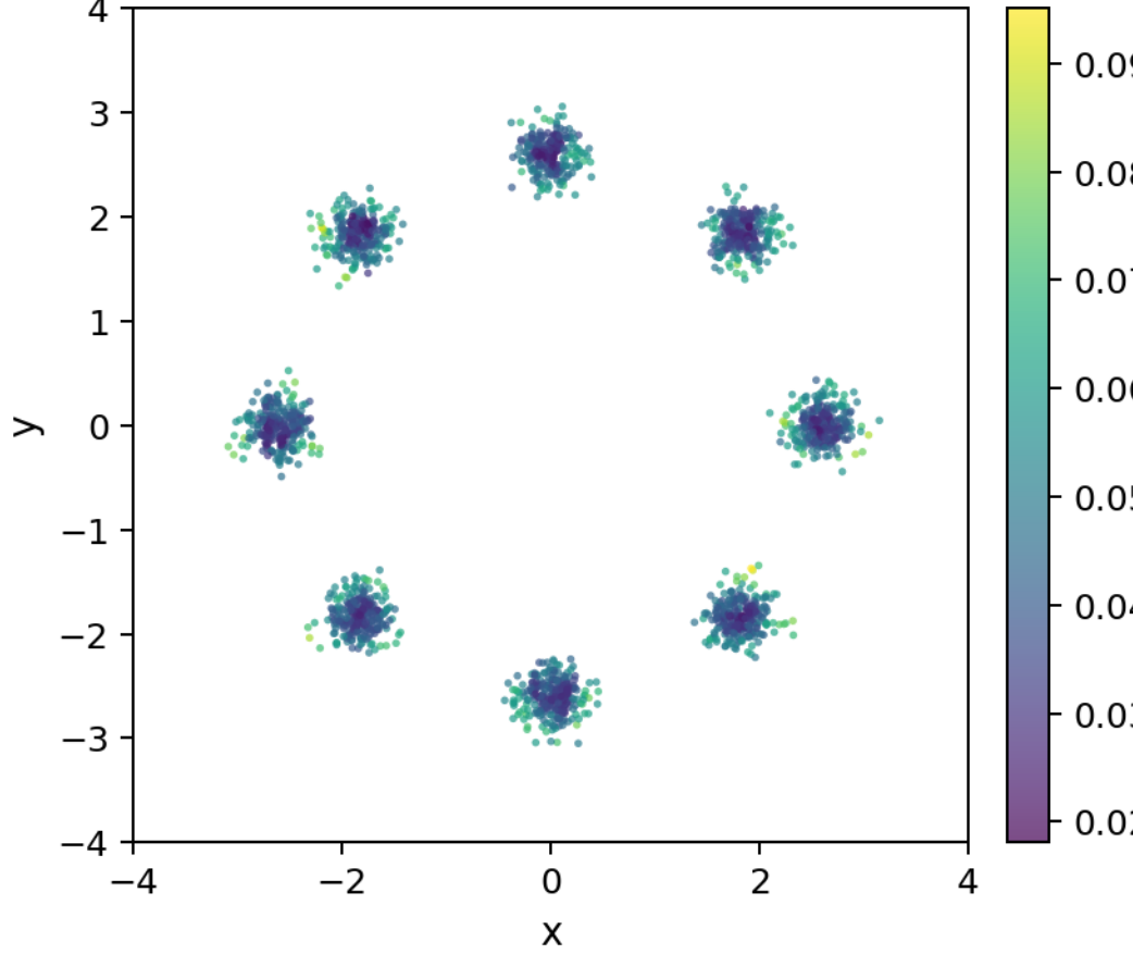
Manifold Thickness
