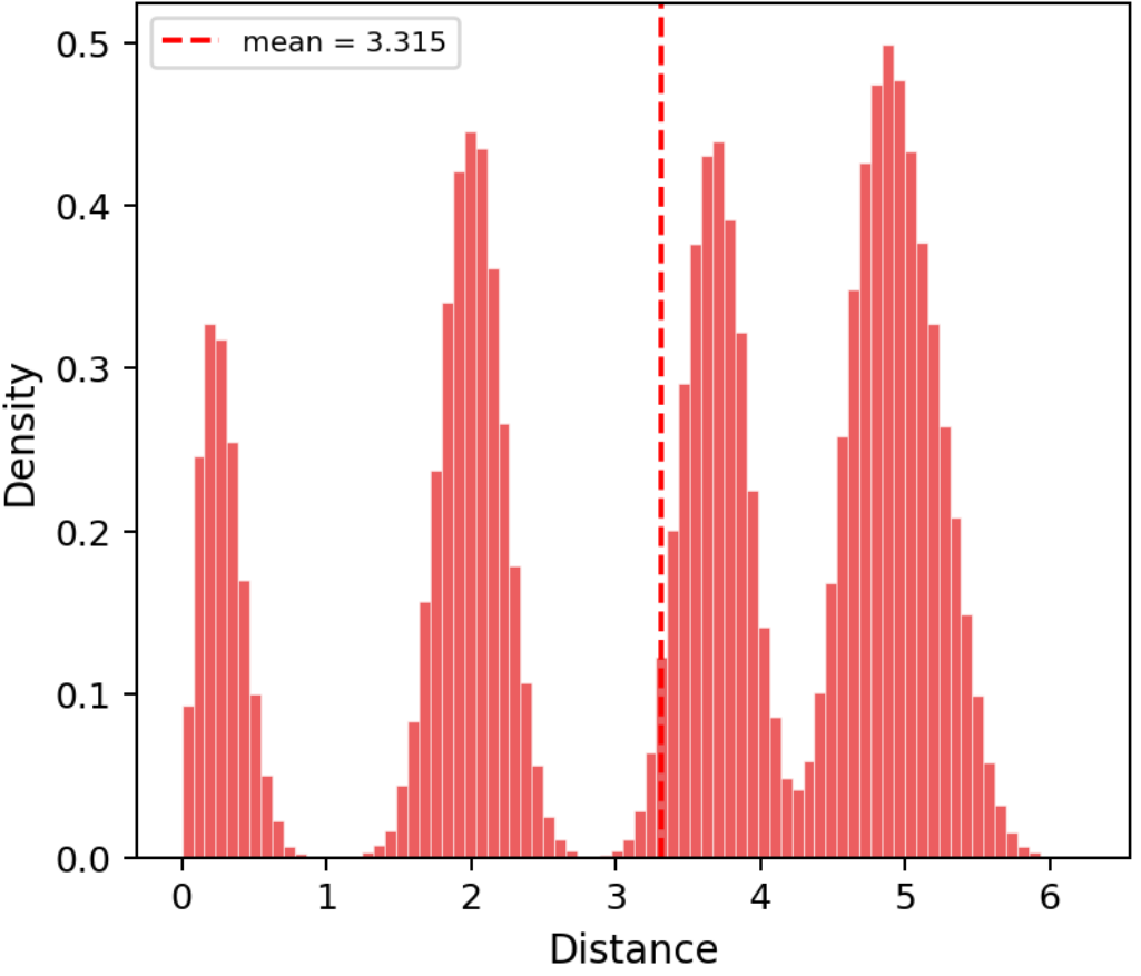
Pairwise Distances
