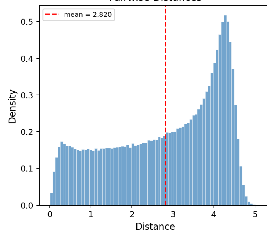
Pairwise Distances
