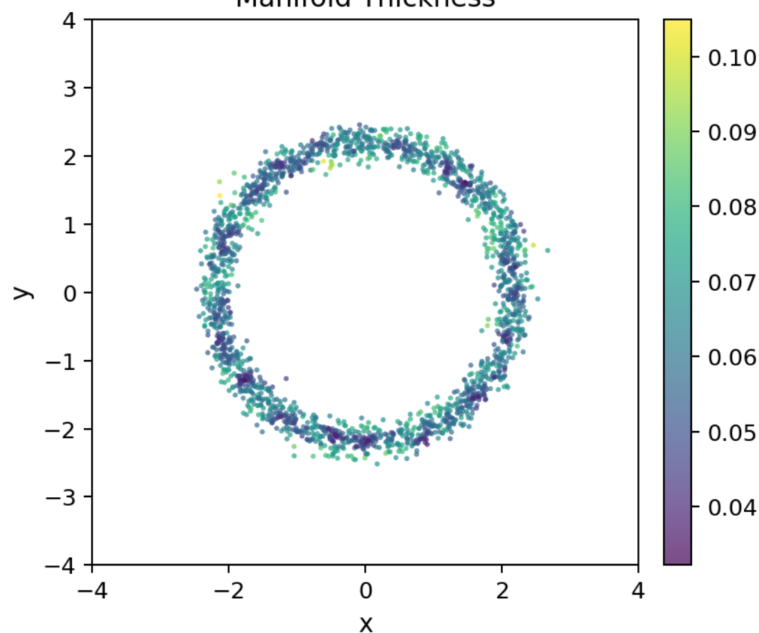
Manifold Thickness
