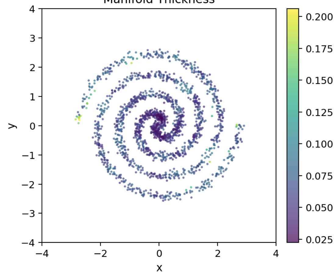
Manifold Thickness
