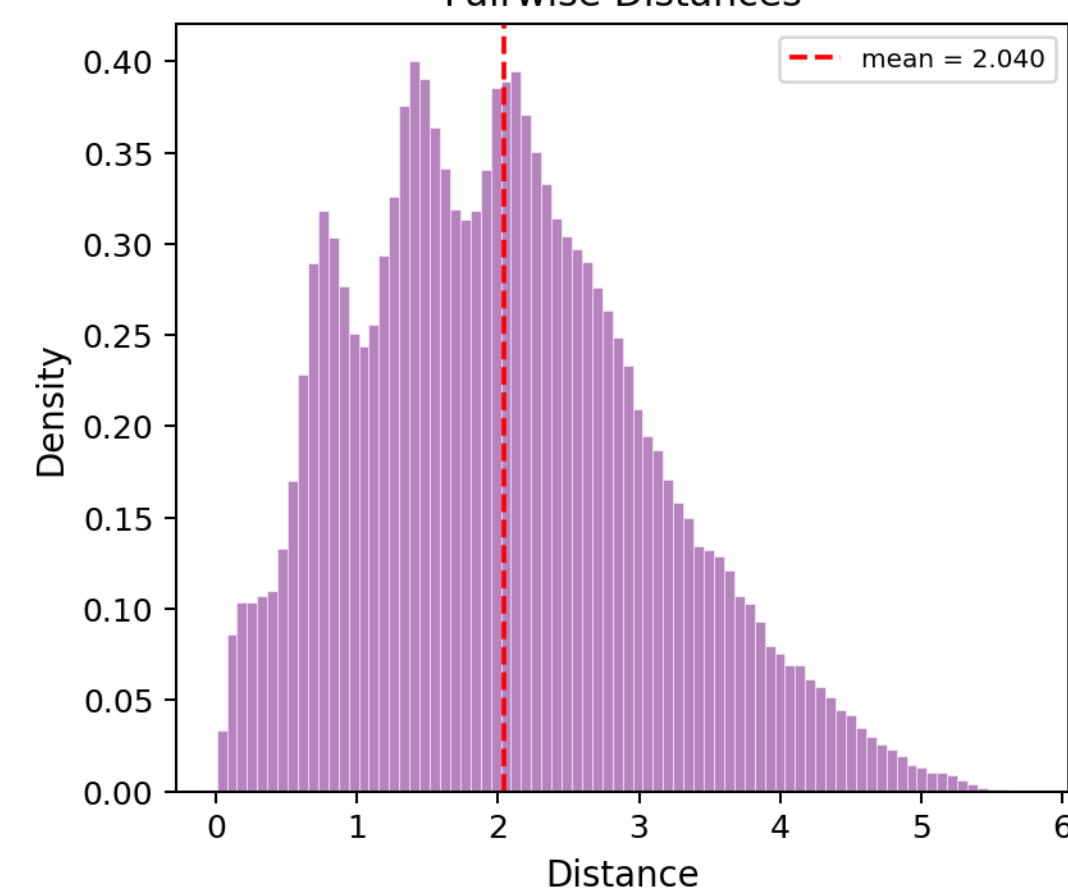
Pairwise Distances
