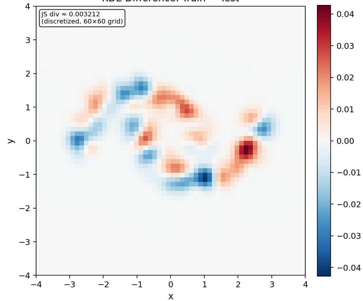
Two Moons KDE Difference: Train – Test
