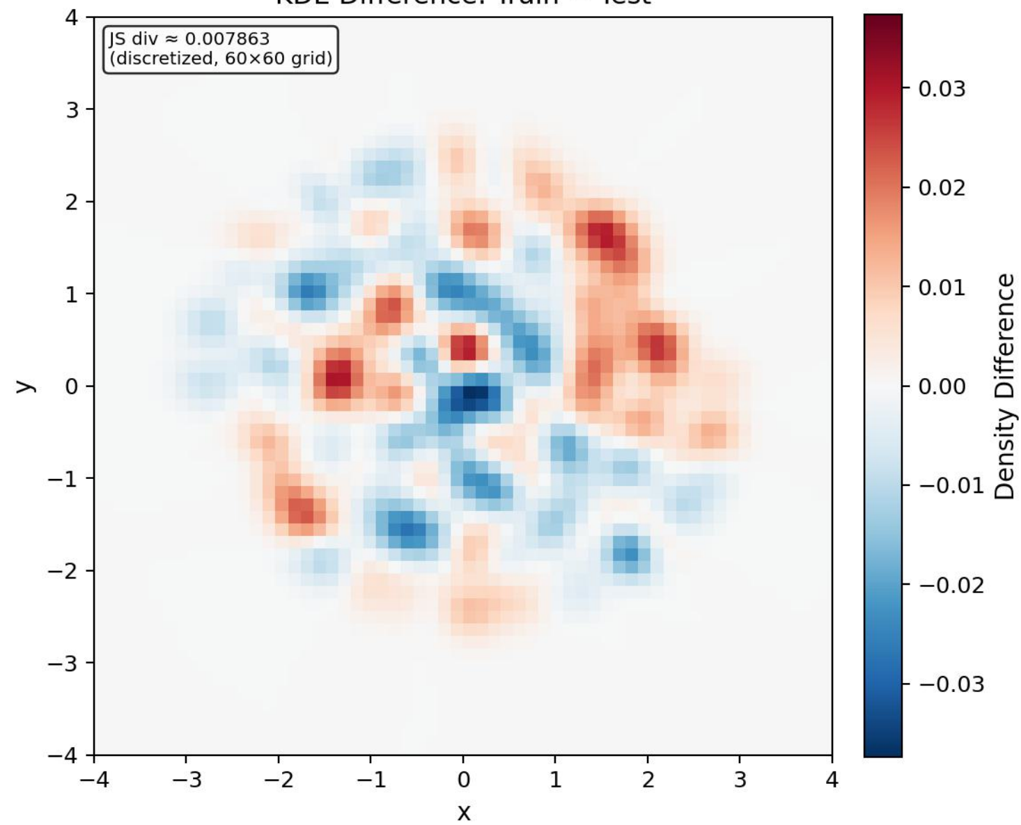
Spiral KDE Difference: Train – Test
