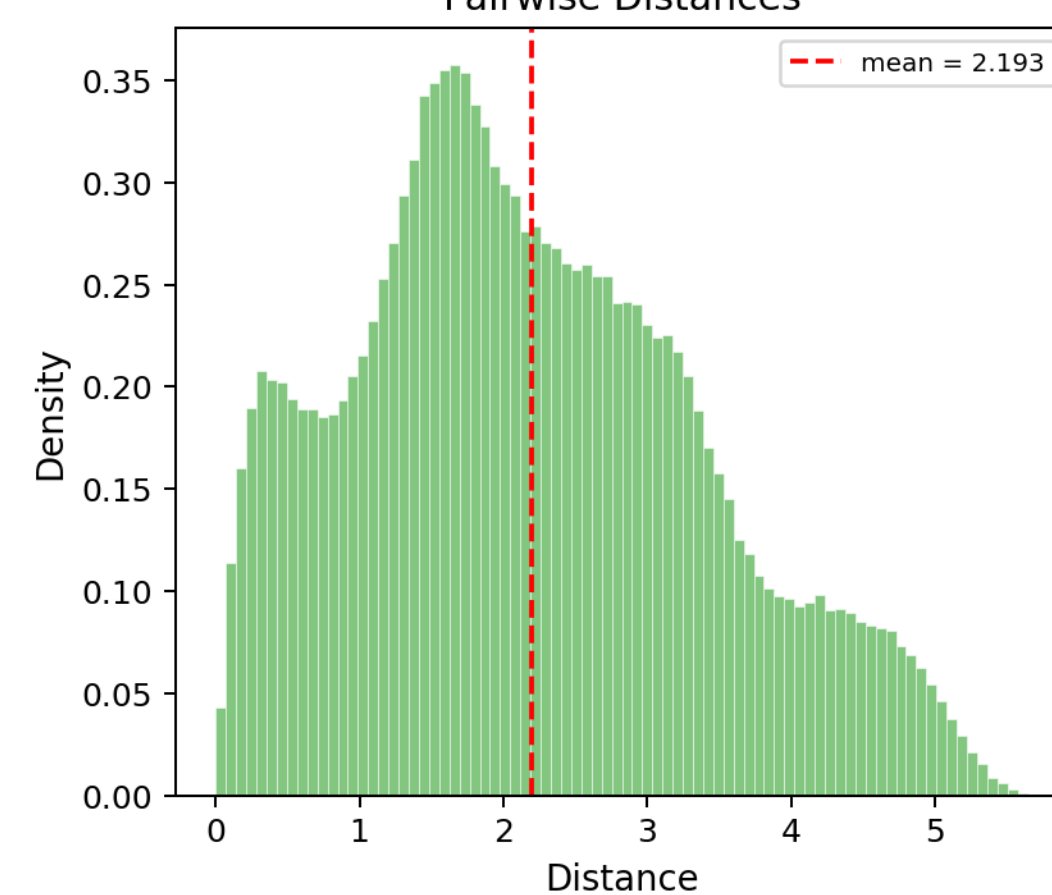
Pairwise Distances
