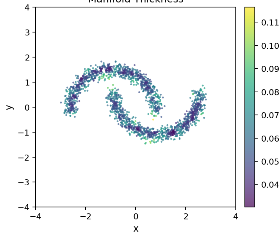
Manifold Thickness
