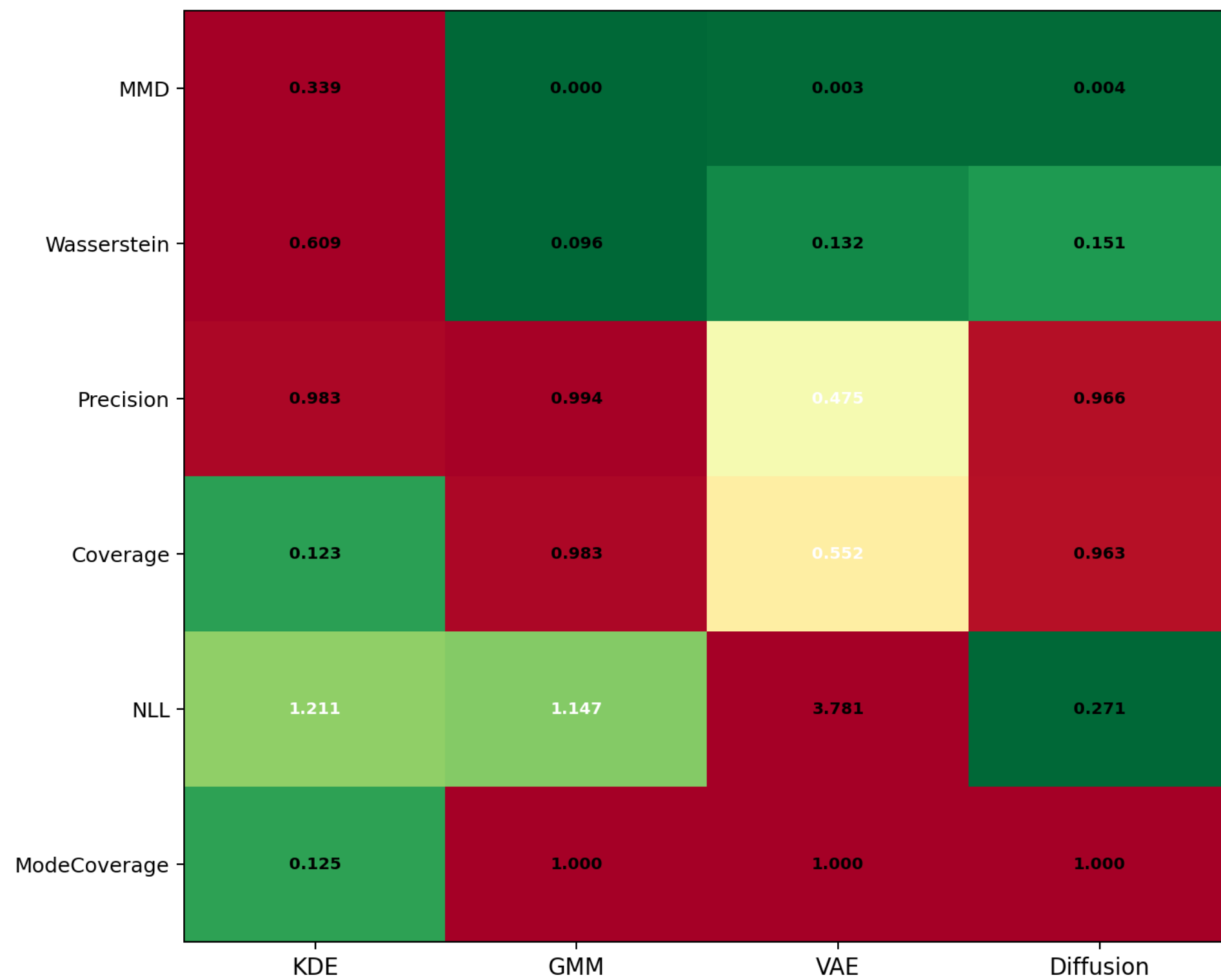
Two Moons
