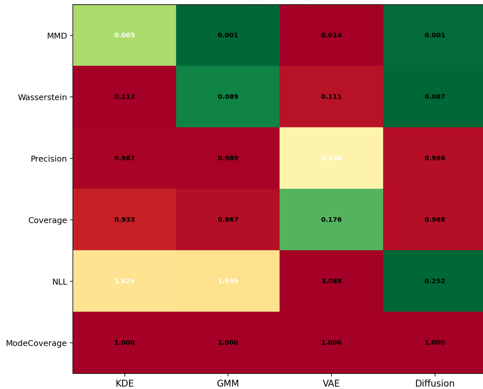
Two Moons
