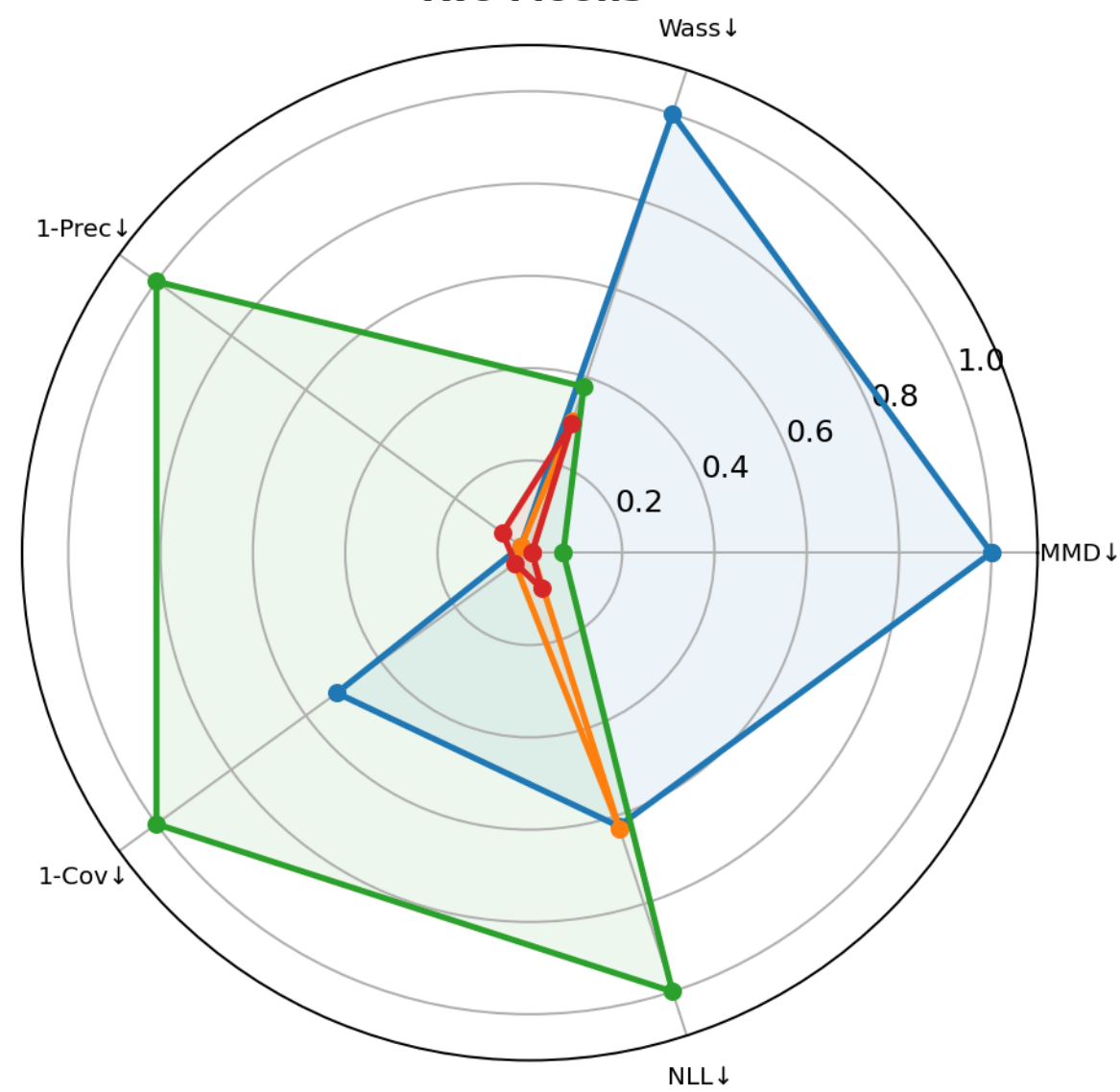
Two Moons
