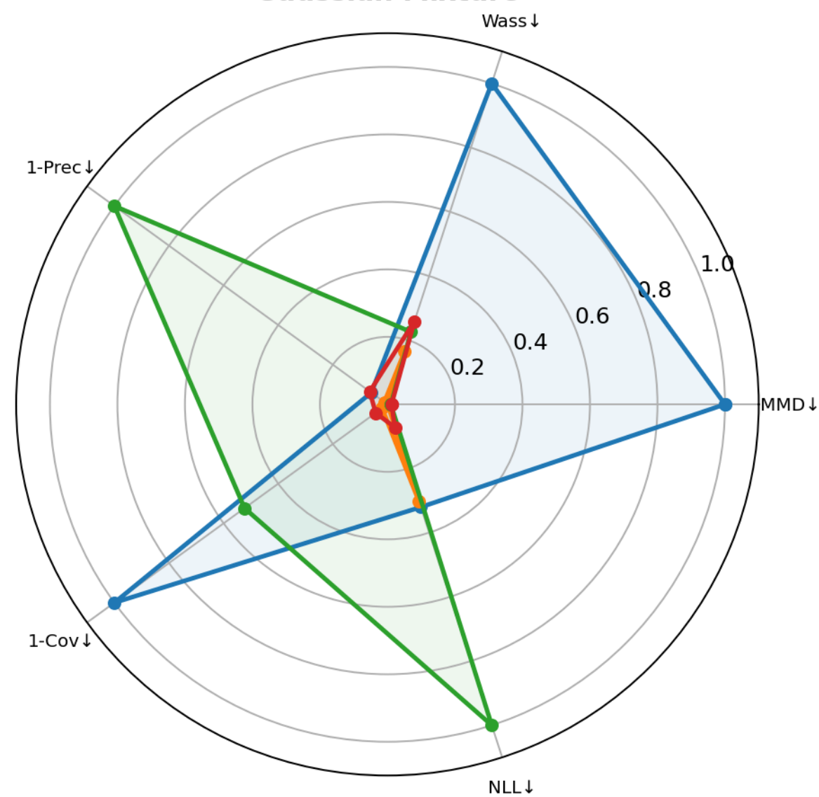
Gaussian Mixture
