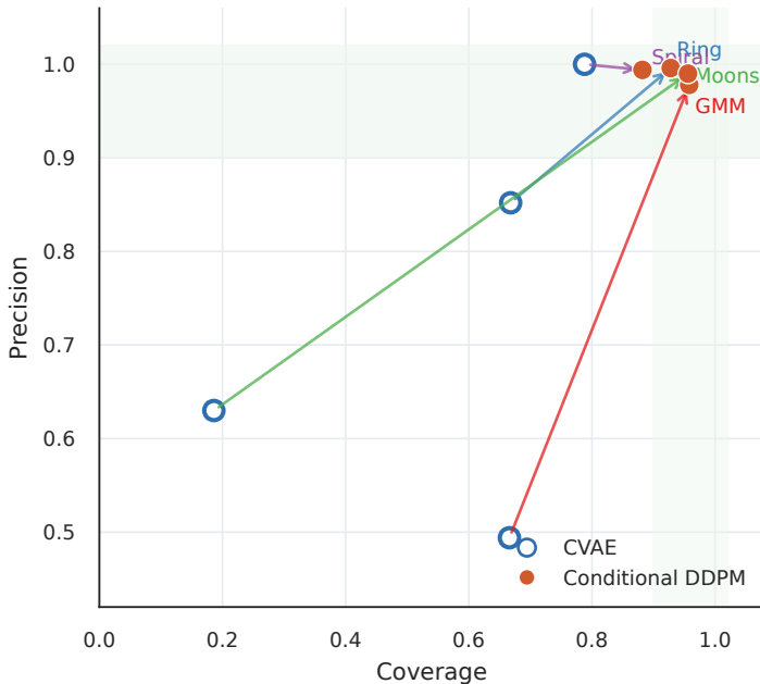
Precision-Coverage plane
