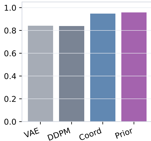
Coverage
