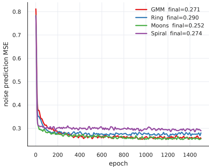
DDPM convergence
