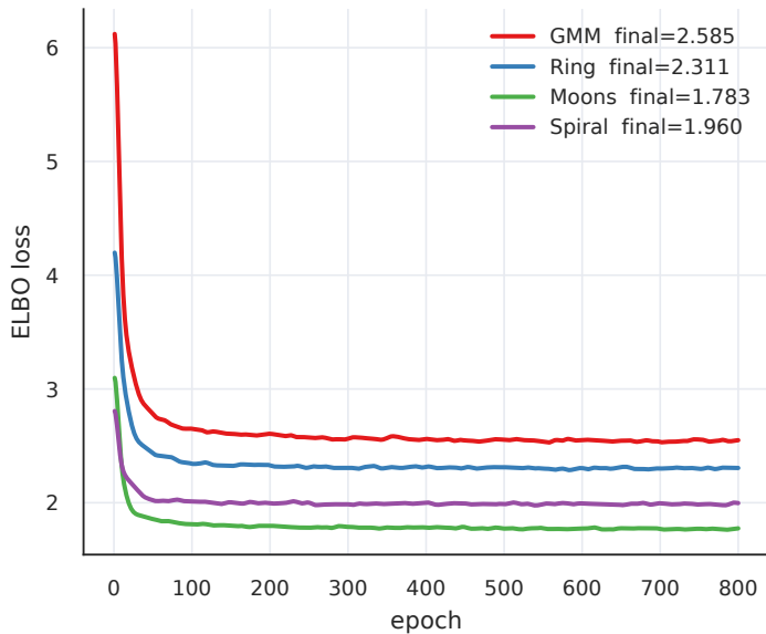
VAE convergence
