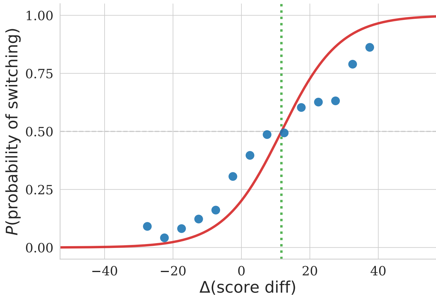
(e) Qwen-72B (\beta = -1.38, \lambda = 0.12)
