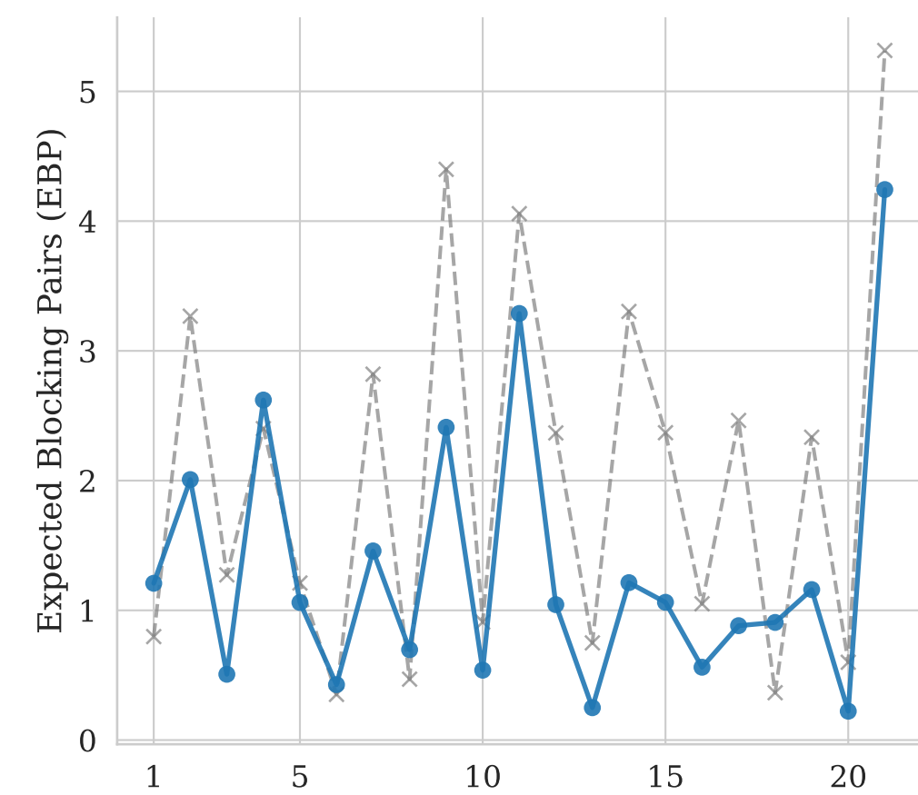
(a) GPT-4-Turbo
