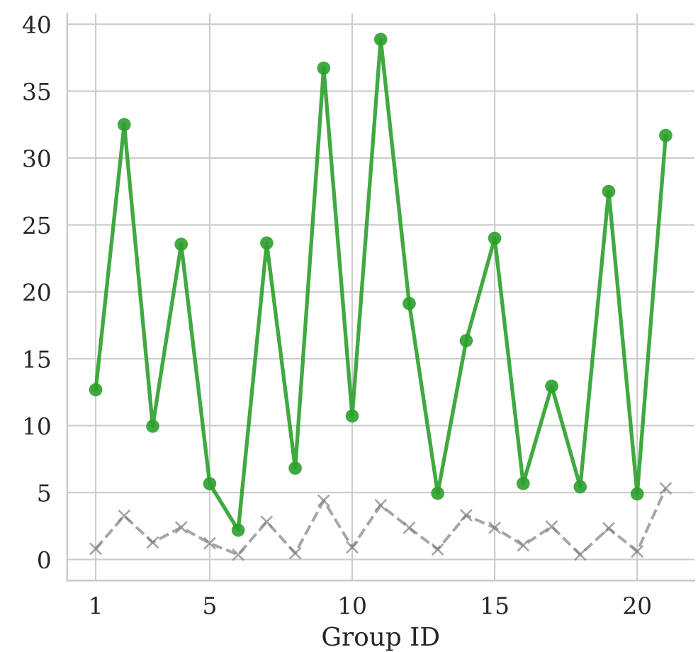
(c) DeepSeek-R1
