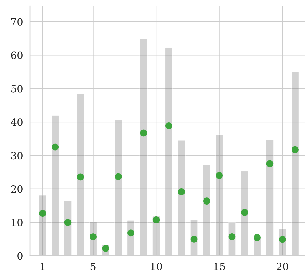
(c) DeepSeek-R1
