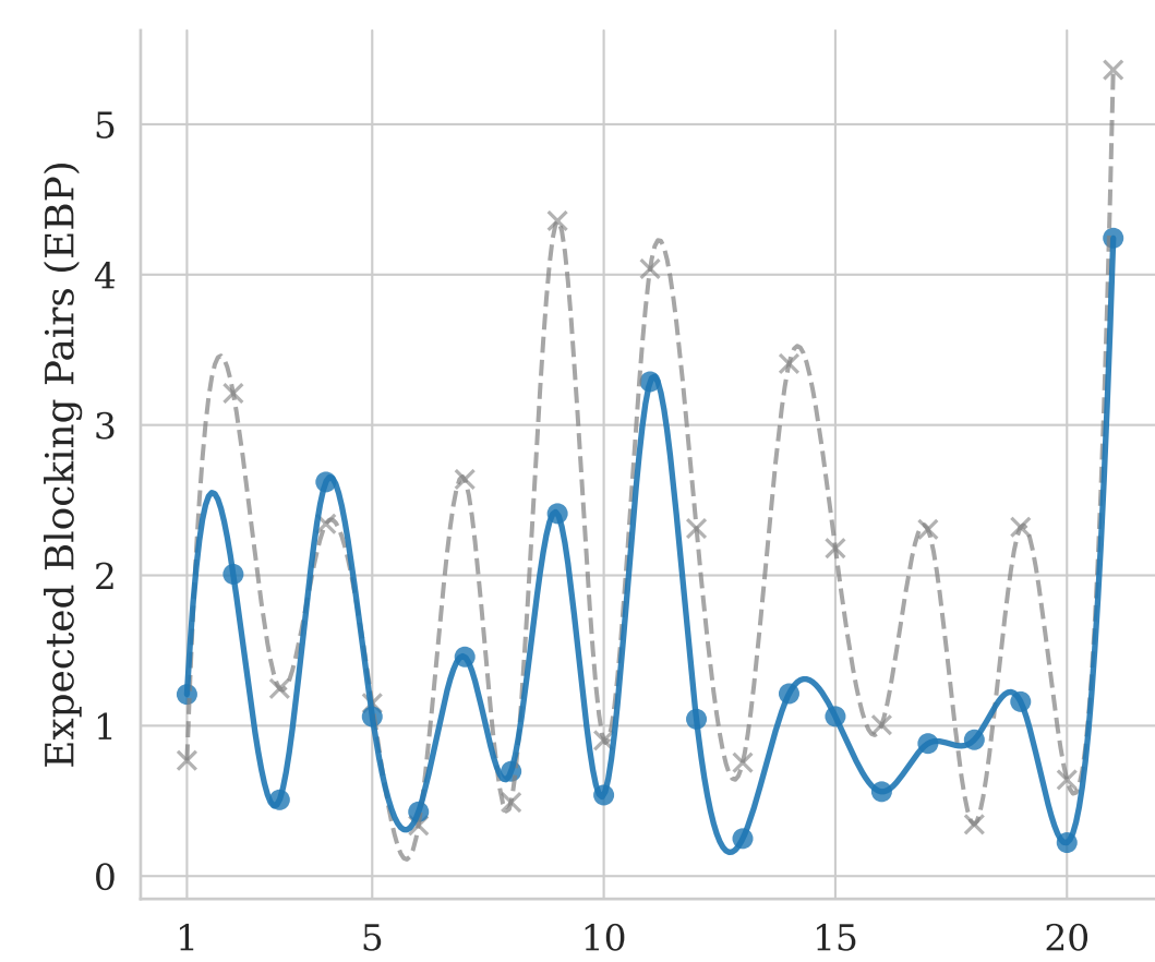
(a) GPT-4-Turbo
