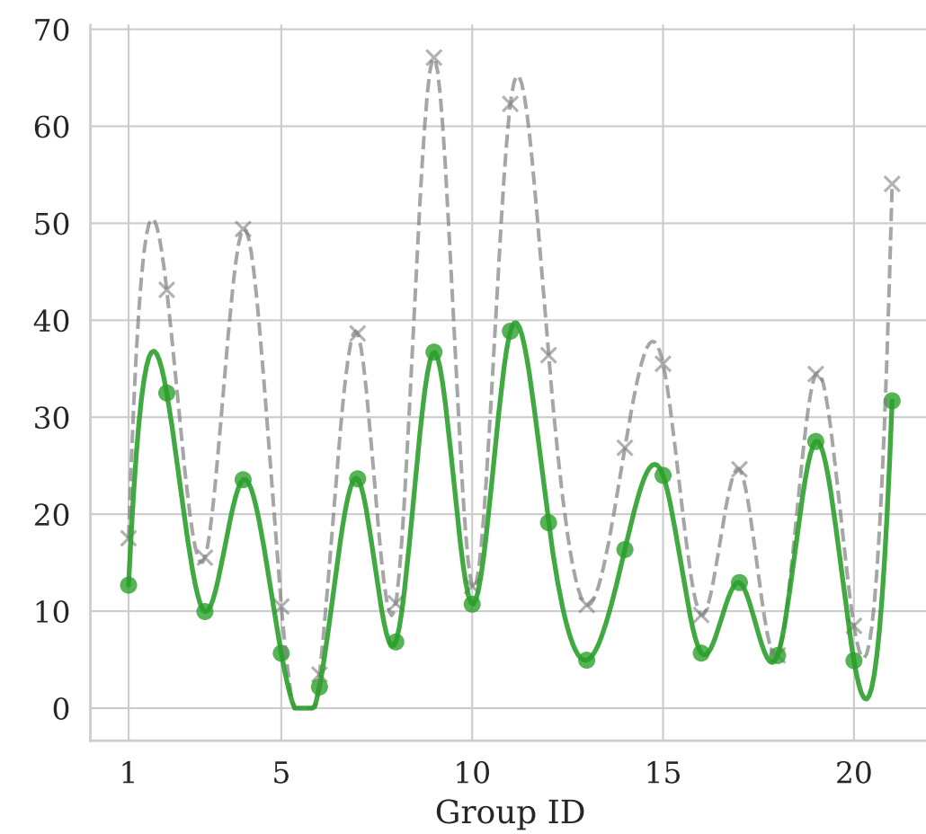
(c) DeepSeek-R1
