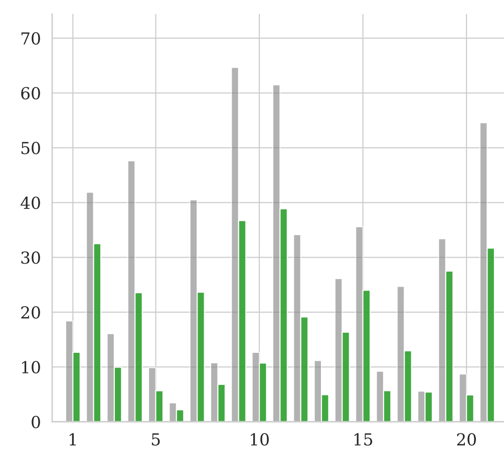
(c) DeepSeek-R1
