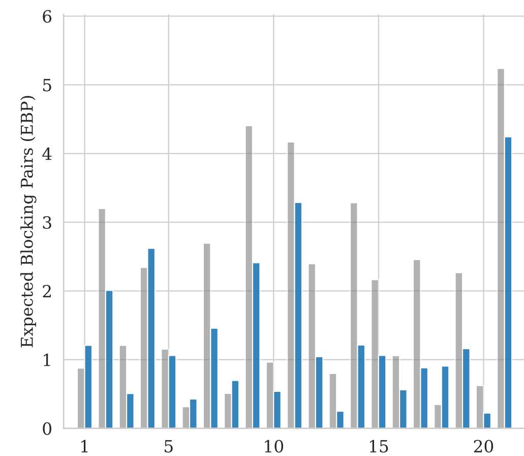
(a) GPT-4-Turbo
