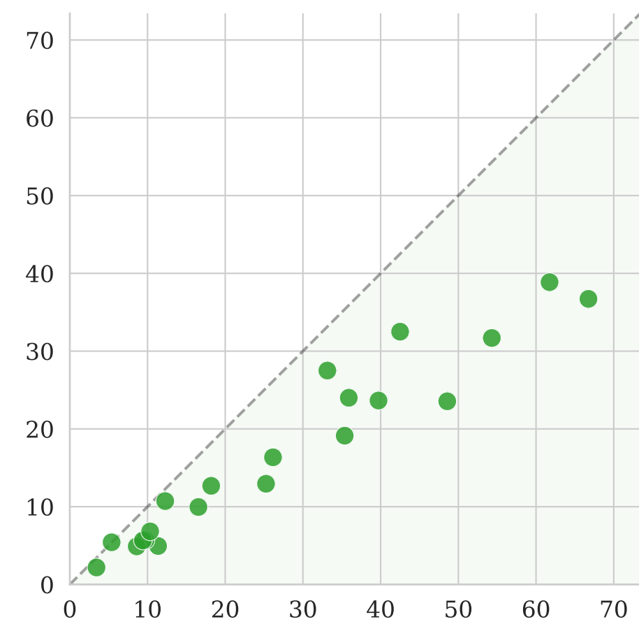
(c) DeepSeek-R1
