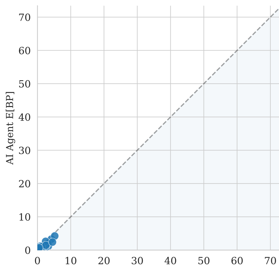
(a) GPT-4-Turbo
