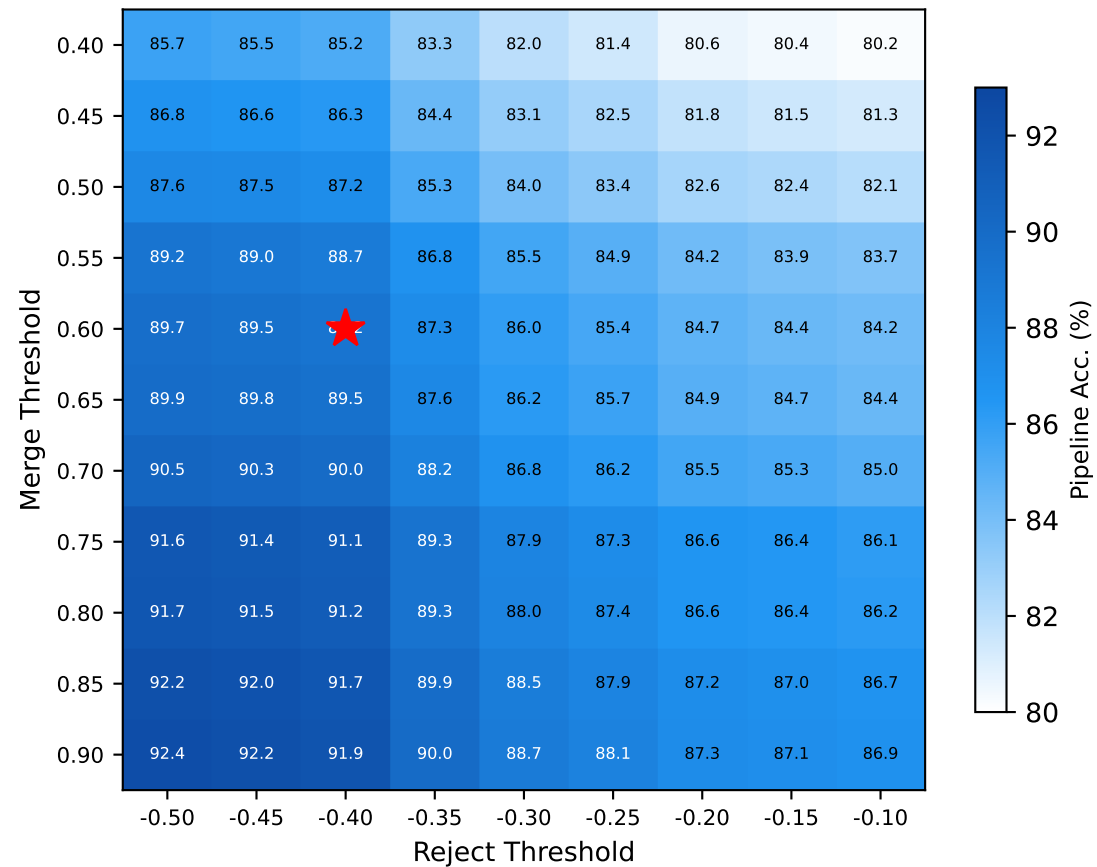
(a) Pipeline Accuracy (%)
