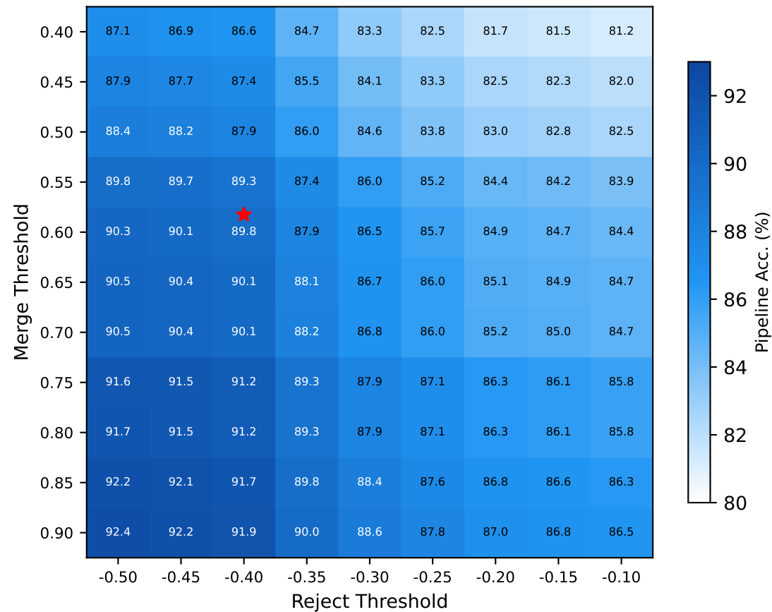
(a) Pipeline Accuracy (%)
