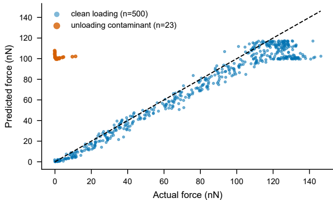
(a) Original (depth-sorted) filter R^2=0.716
