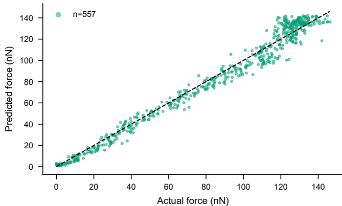
(b) Corrected (time-ordered) filter R^2=0.975
