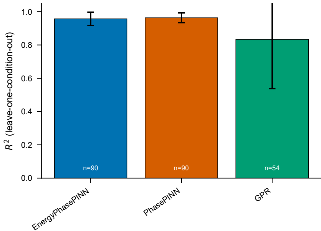
Model comparison (mean \pm SD across folds/seeds)
