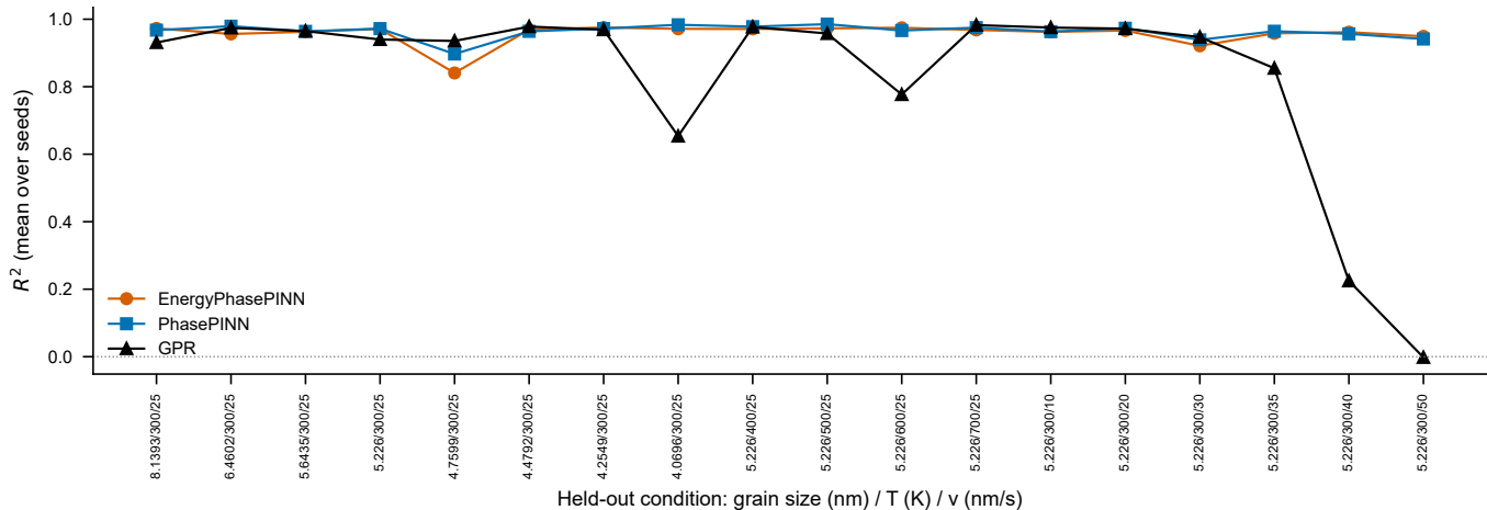
Per-condition reliability: GPR degrades at design extremes; both PINNs stay robust
