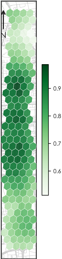
Daily-life sufficiency (Moran I=0.932)
