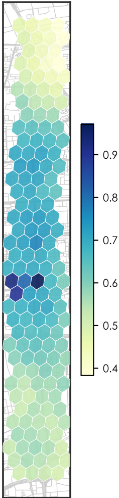
AI industry suitability (Moran I=0.874)
