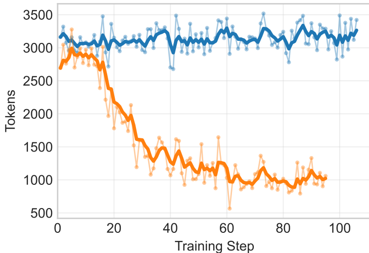
Code Executor Response Length
